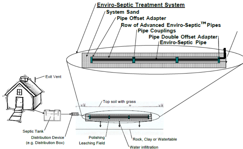
Diagram of the Enviro-Septic system
